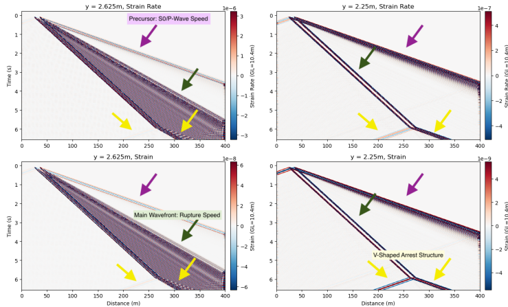
Figure: Horizontal Strain and strain rate for sub-Rayleigh crack propagation in simple two-layer model. Plotted at crack depth ( 2.625\text{m} ) and at the snow bottom ( 2.25\text{m} ). Gauge length is 10.4\text{m} .
