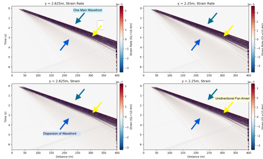
Figure: Horizontal Strain and strain rate for Supershear crack propagation in simple two-layer model. Plotted at crack depth (2.625m) and at the snow bottom (2.25m). Gauge length is 10.4m.
